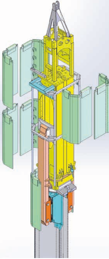
HAMMER NOISE REDUCTION (EXPLODED VIEW)
